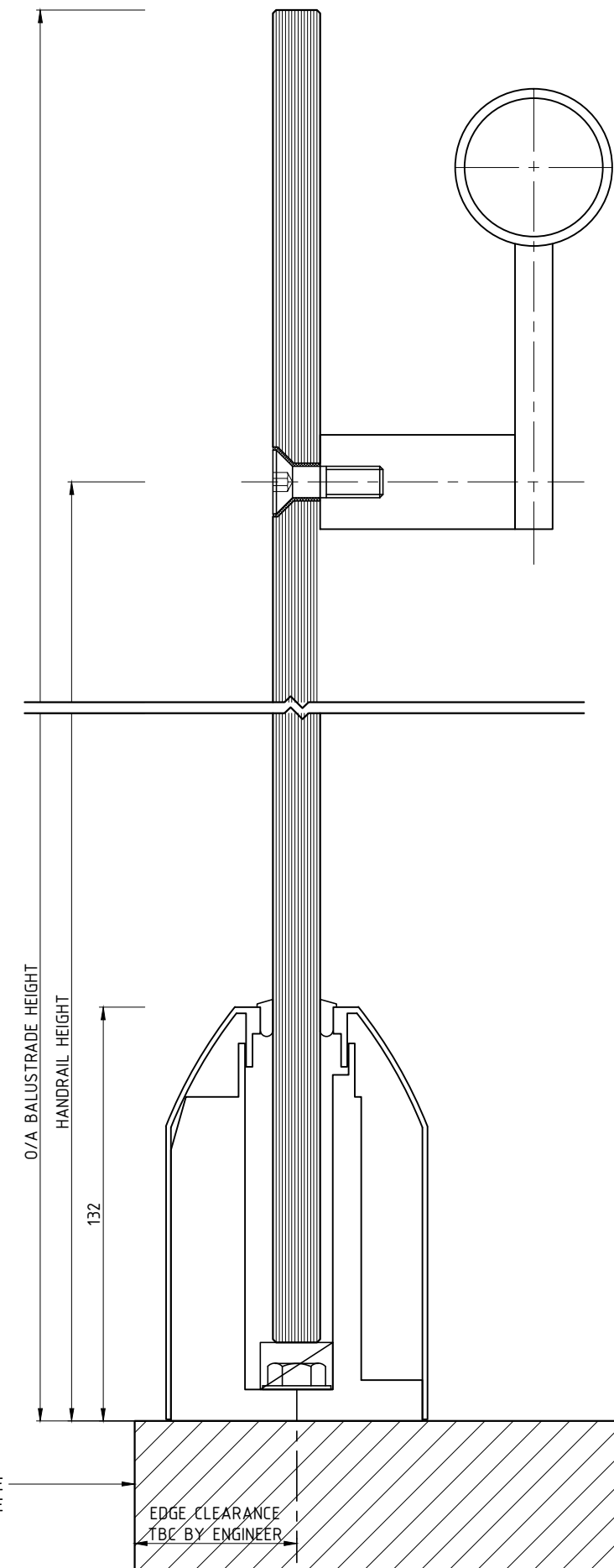
02 01 HANDRAIL DETAIL 1:2
