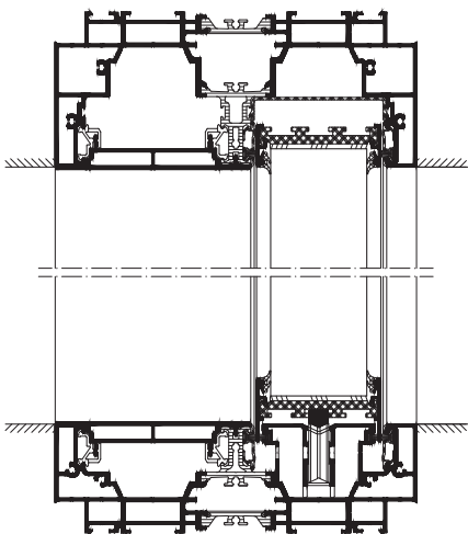
Example: Access Line level threshold
