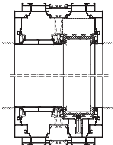
Example: Design Line frameless view
