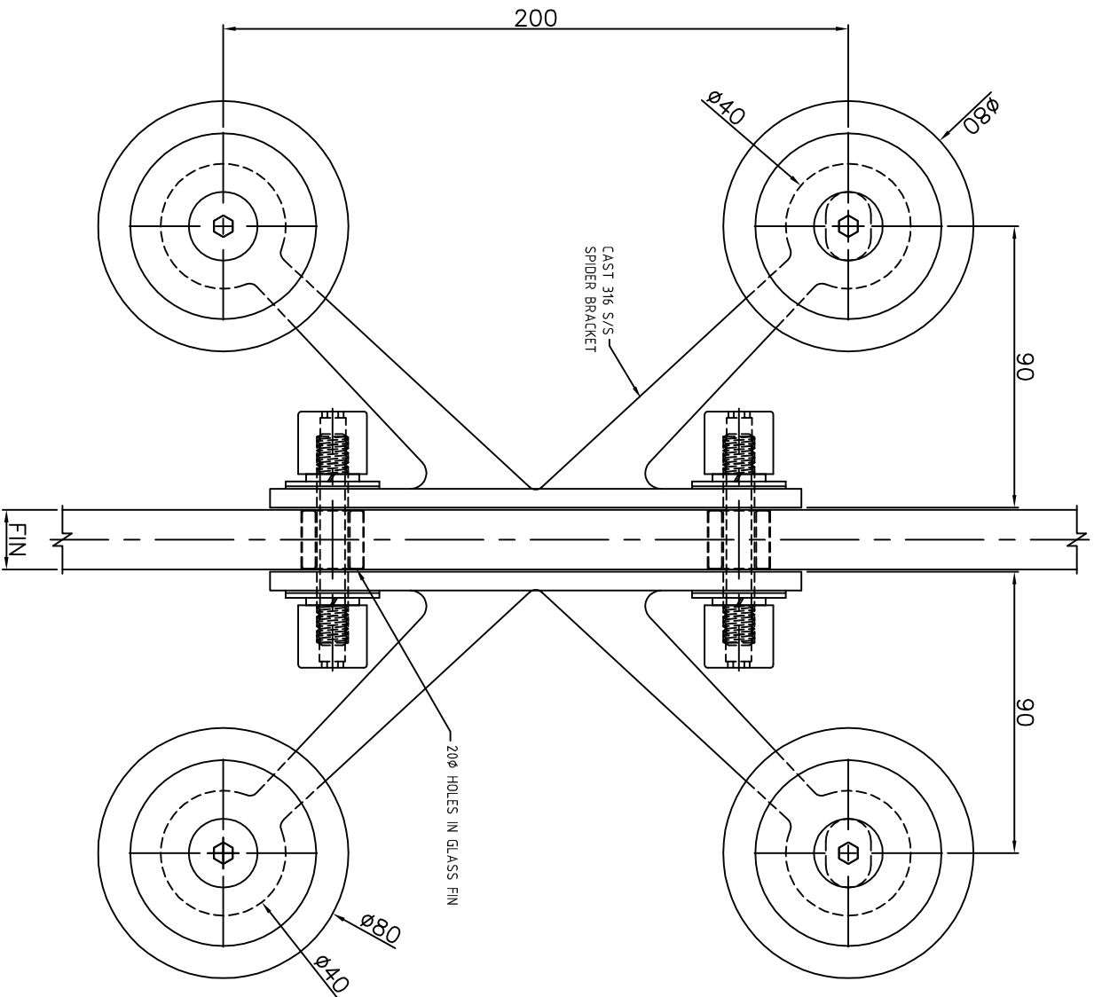
4 WAY 'GLASS FIN' SPIDER
