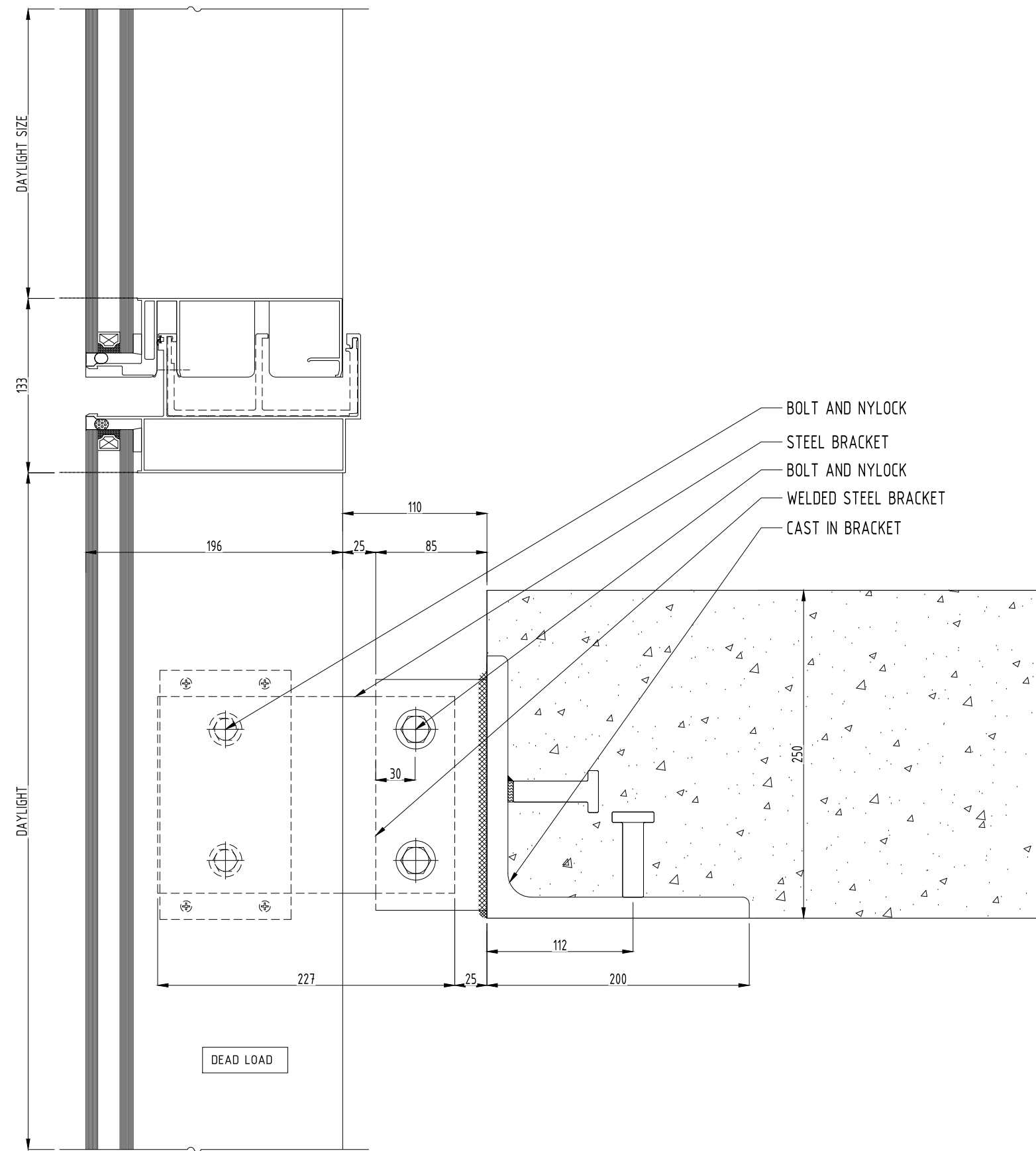
BRACKET SECTION DETAIL 02 01 1:2
