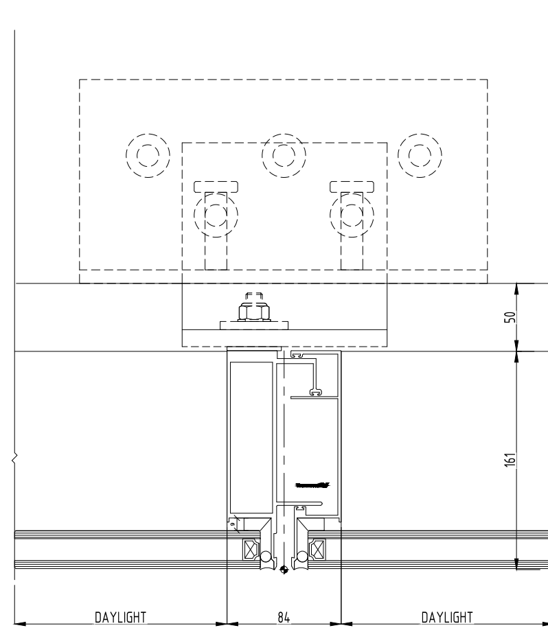
01 01 BRACKET PLAN DETAIL 1:2
