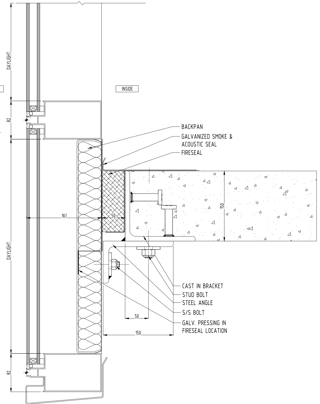
02 01 BRACKET SECTION DETAIL 1:2
