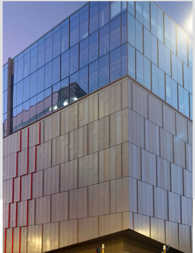
The National Archives Heke Rua building in Wellington - features a Thermosash PW1000 Thermally Broken unitised curtainwall compliant with BS/EU 16893 - a factor of 10 better air infiltration / ex-filtration than NZS4284 compliance.
