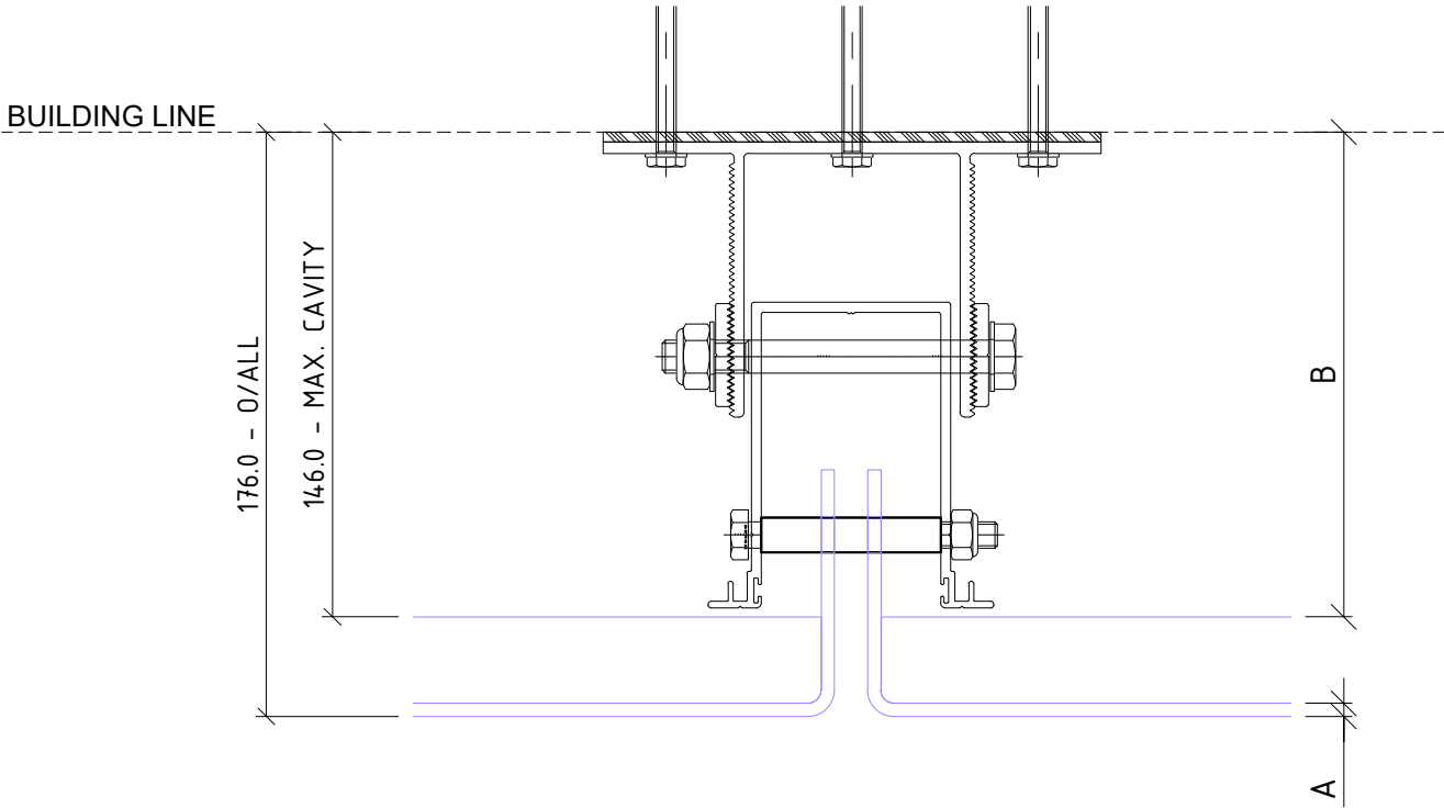
EN05 - FF MAXIMUM SYSTEM CAVITY 146mm
