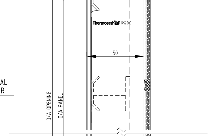
STANDARD HORIZONTAL DETAIL 03/01 1:2
