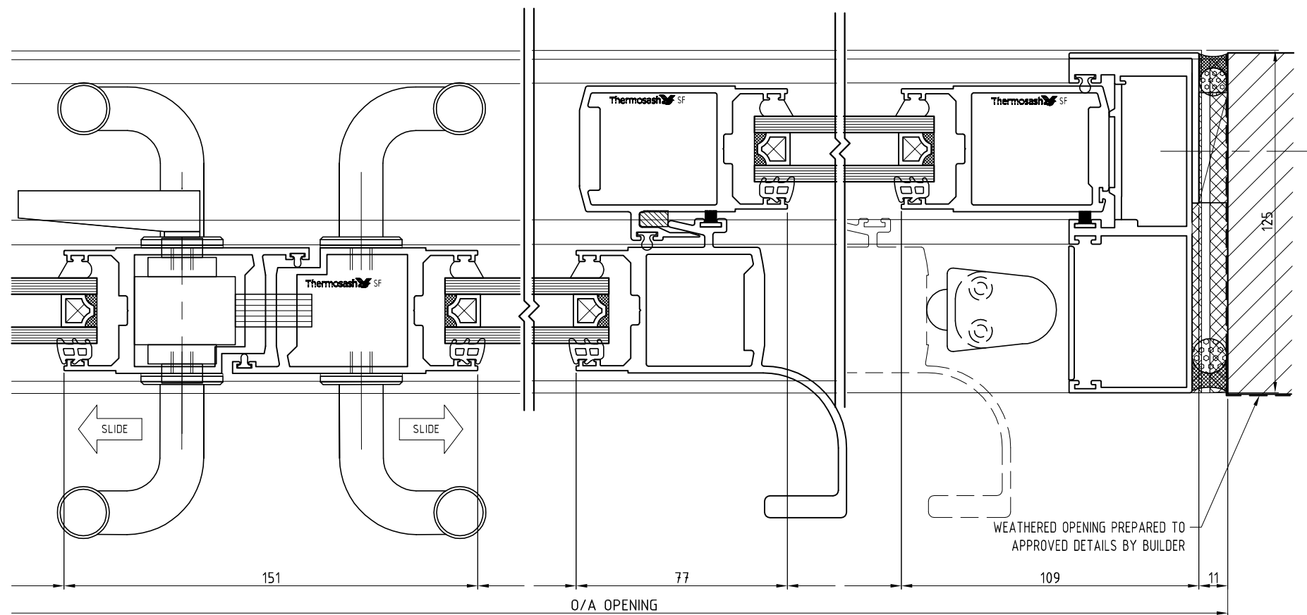
05 04 SLIDER PARTING 1:2
