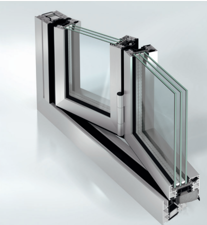
Schüco AS FD 90.HI (continuous outer frame, inward or outward-opening)
