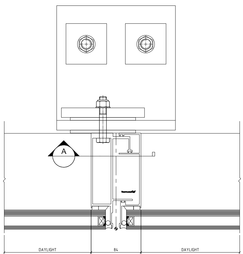
01 01 BRACKET PLAN DETAIL 1:2
