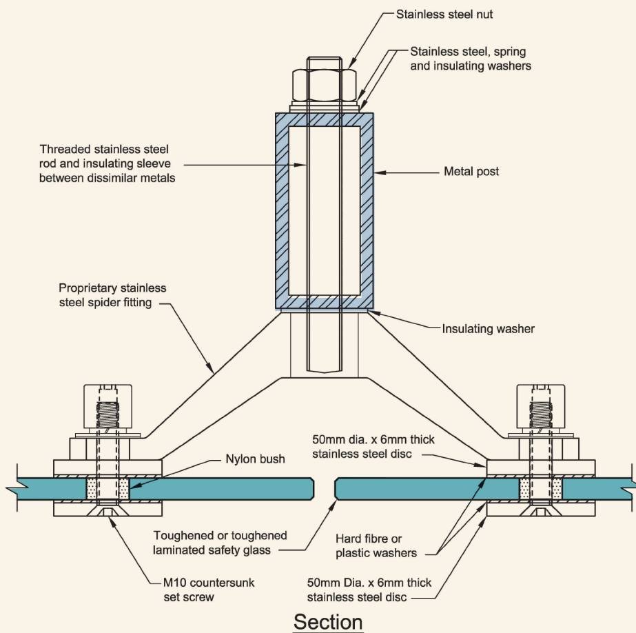
Figure 4.4 Glass fixed with spider fitting to post
