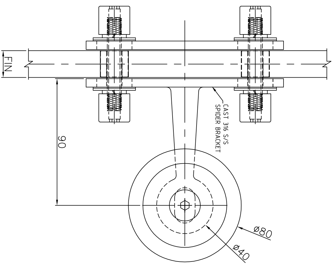
SINGLE 'GLASS FIN' SPIDER
