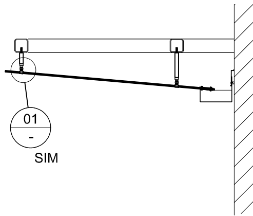
B - SECTION
